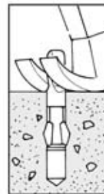
Insert anchor. Expand by hammer.
